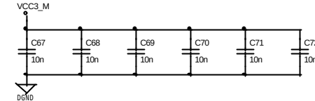
SGRAM DECOUPLING CAPACITORS
