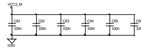
SGRAM DECOUPLING CAPACITORS
