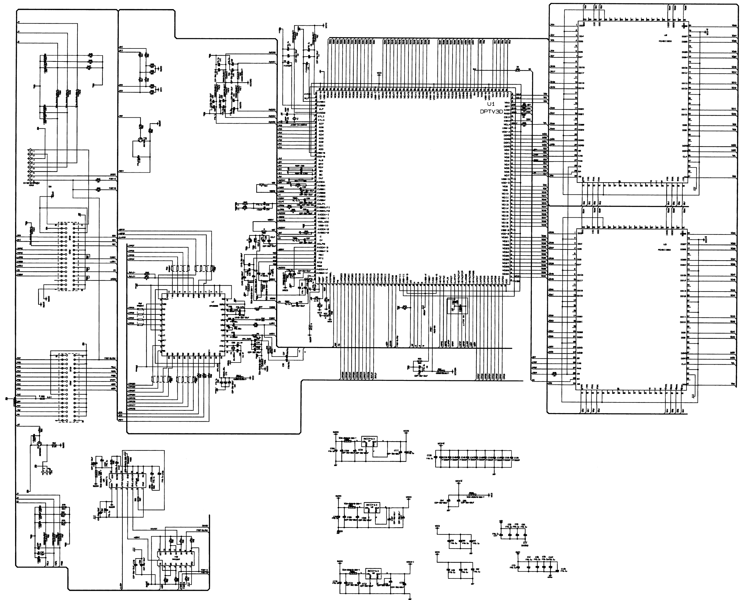
DPTV BOARD
