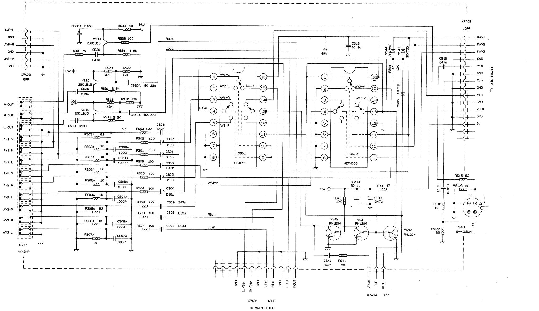
Power Board JU7. 820. 1587
