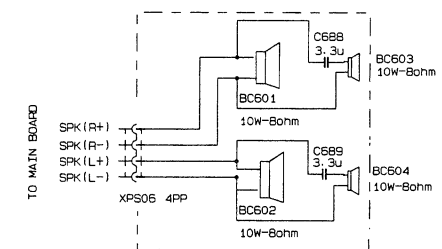
Speaker
