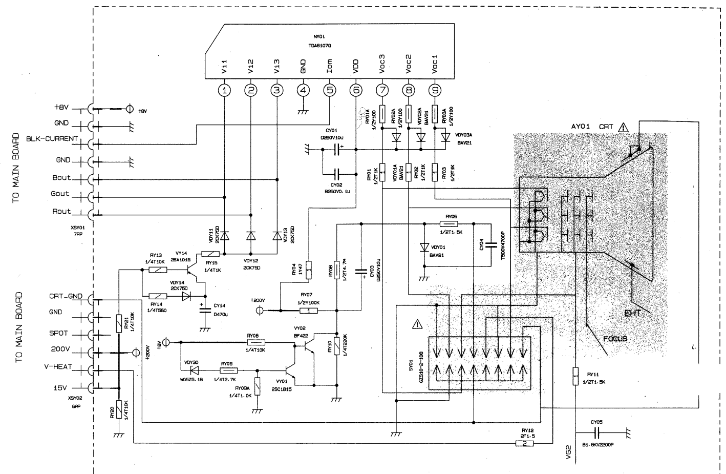
Y BOARD JU7.820.1586-2
