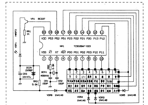
Remote Board JU7.820.1529
