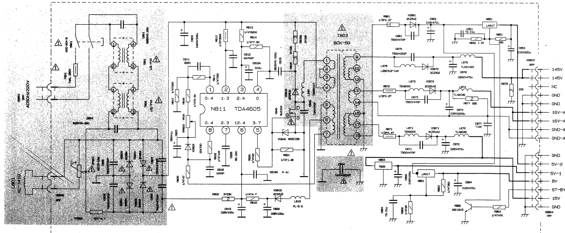
POWER BOARD JU7.820.1587-2
