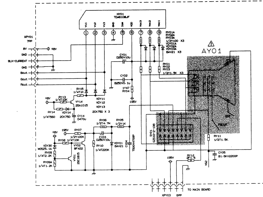
Y Board JU7.820.1586-1
