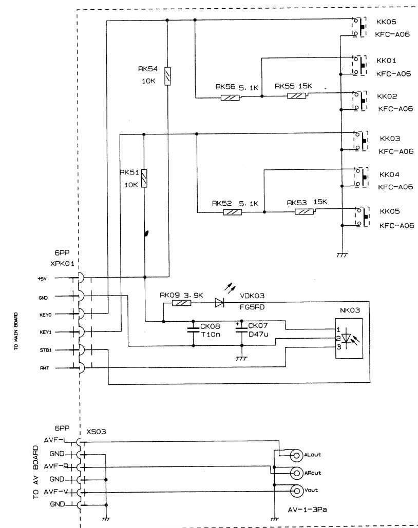
K Board JU7.820.1820
