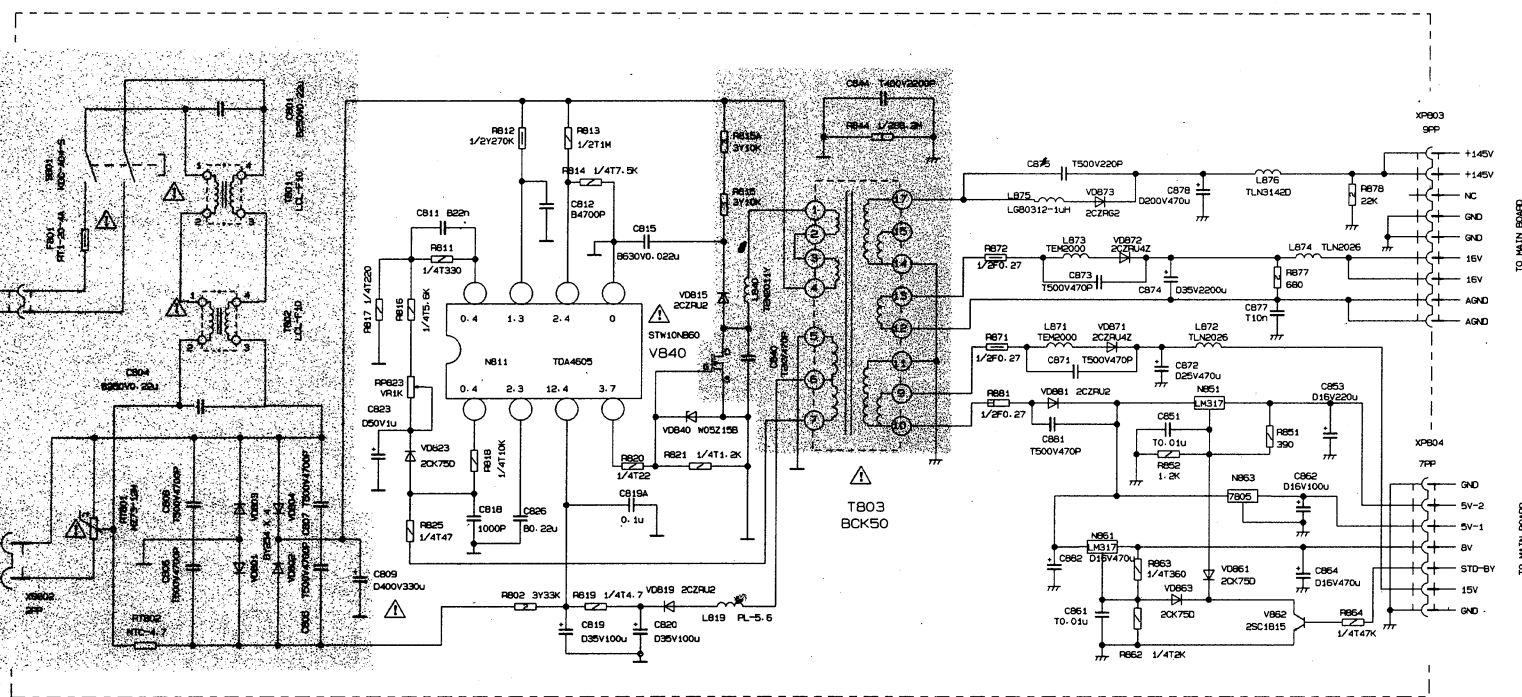
Power Board JU7.820.1587
