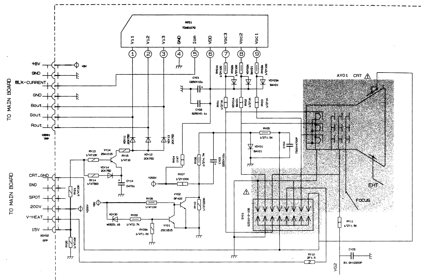
Y BOARD JUC7.820.029
