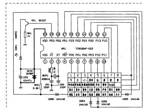
Remote Board JU7.820.1529
