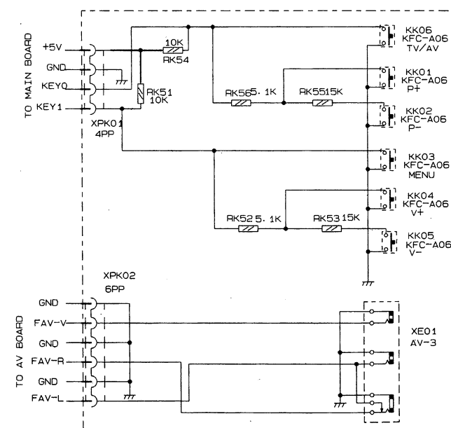
K BOARD JUC7.820.027
