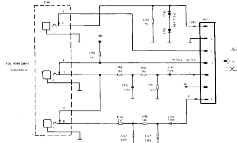
HEADPHONE PANEL
