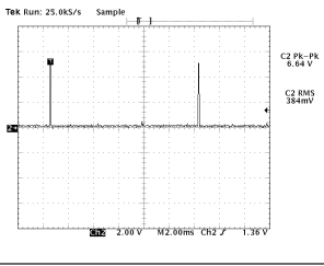
19 2.00 V (IC104, #10)
